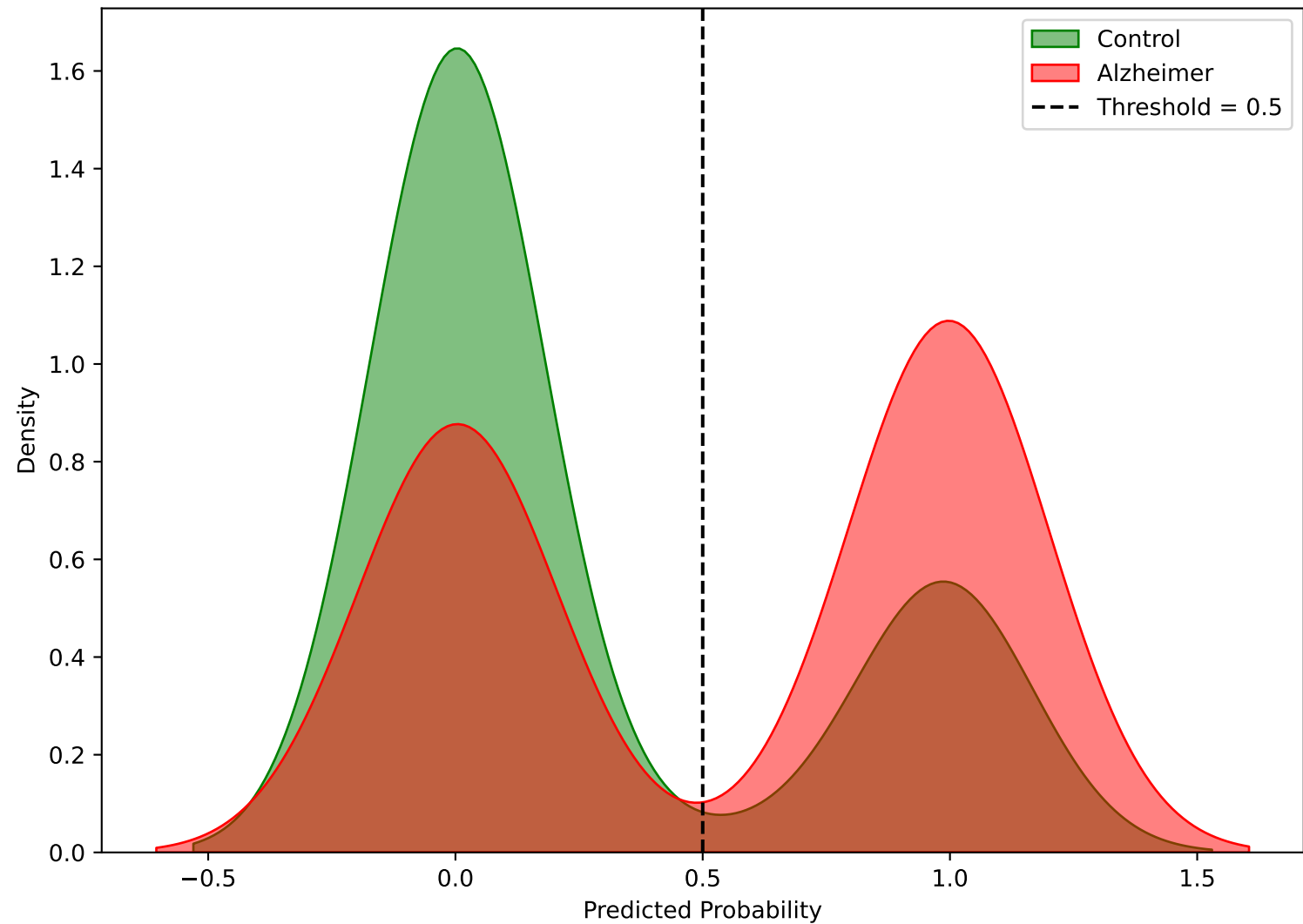
Risk Score Distribution - GaussianNB
